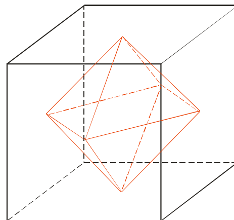
Octahedron, dual of the Cube
